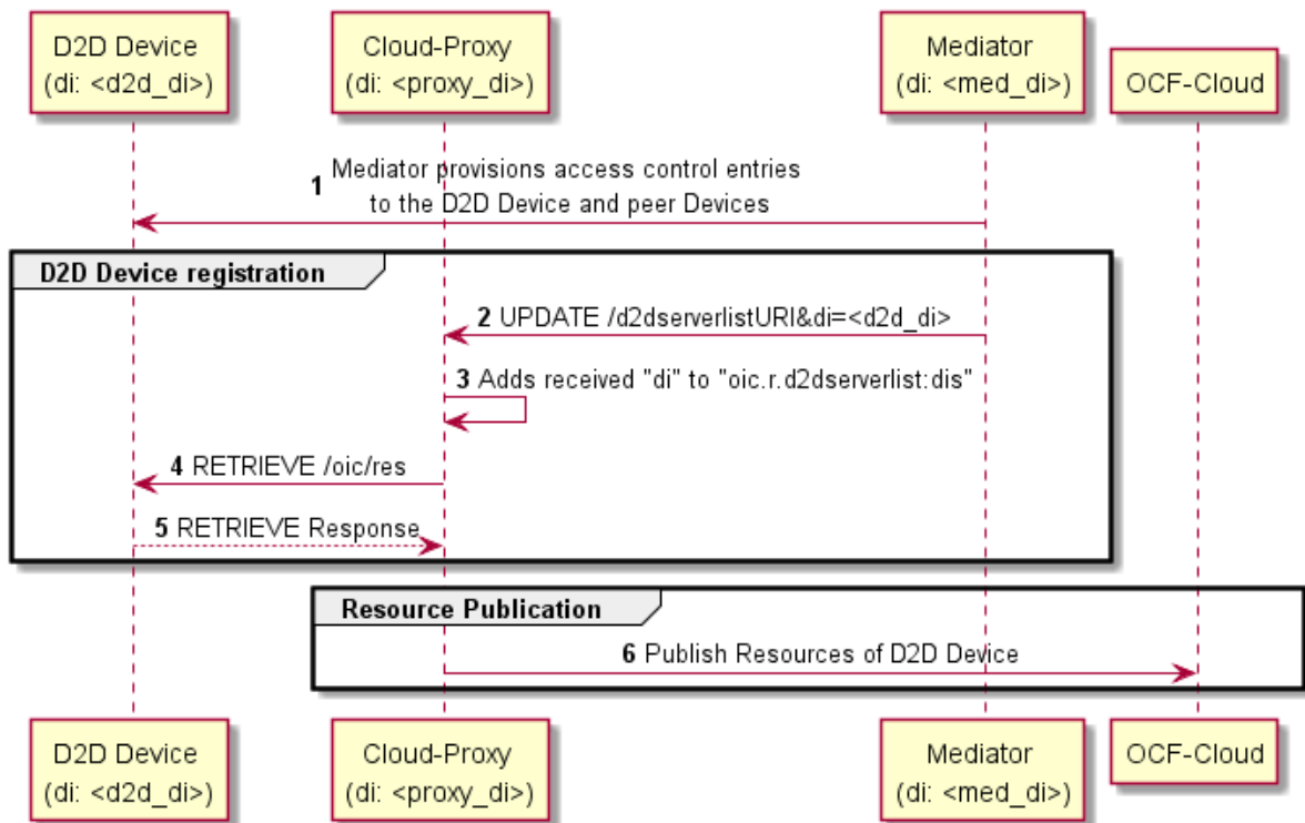
Figure 15 – Resource publication to the OCF Cloud
