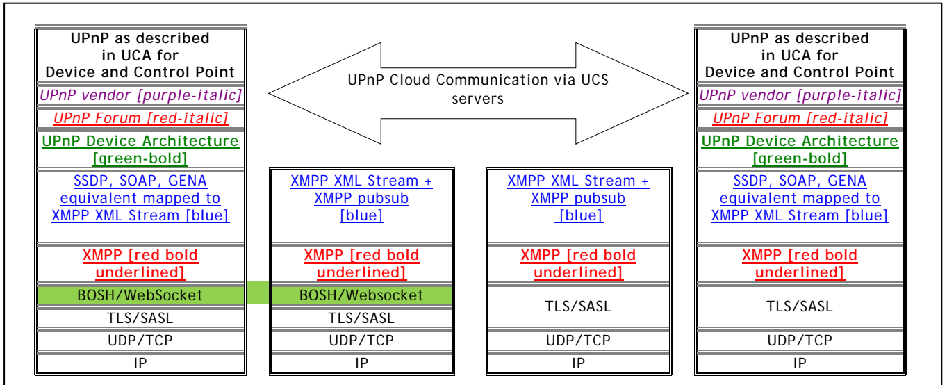
Figure C-12: — BOSH and WebSocket at UCA component stacks
