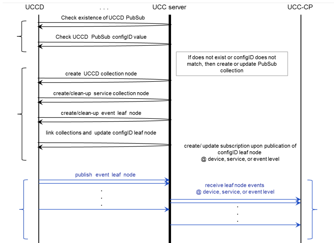
Figure C-10: — PubSub Hierarchy Event Structure Creation
