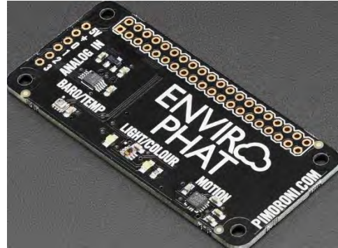
Environment sensors
